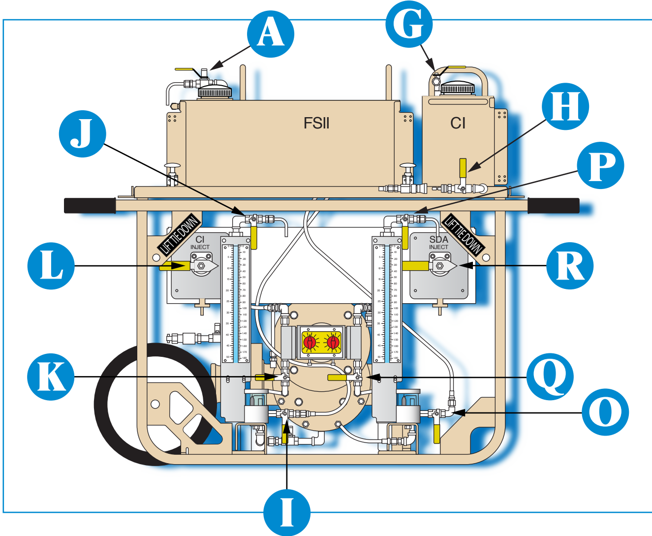
Figure #7–CI/SDA side VALVE IDENTIFICATION
