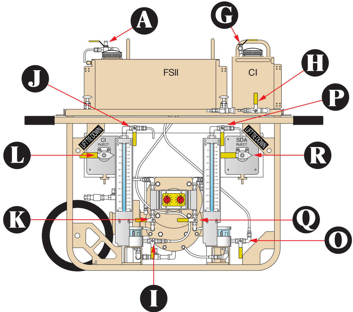
Figure #7–CI/SDA side VALVE IDENTIFICATION
