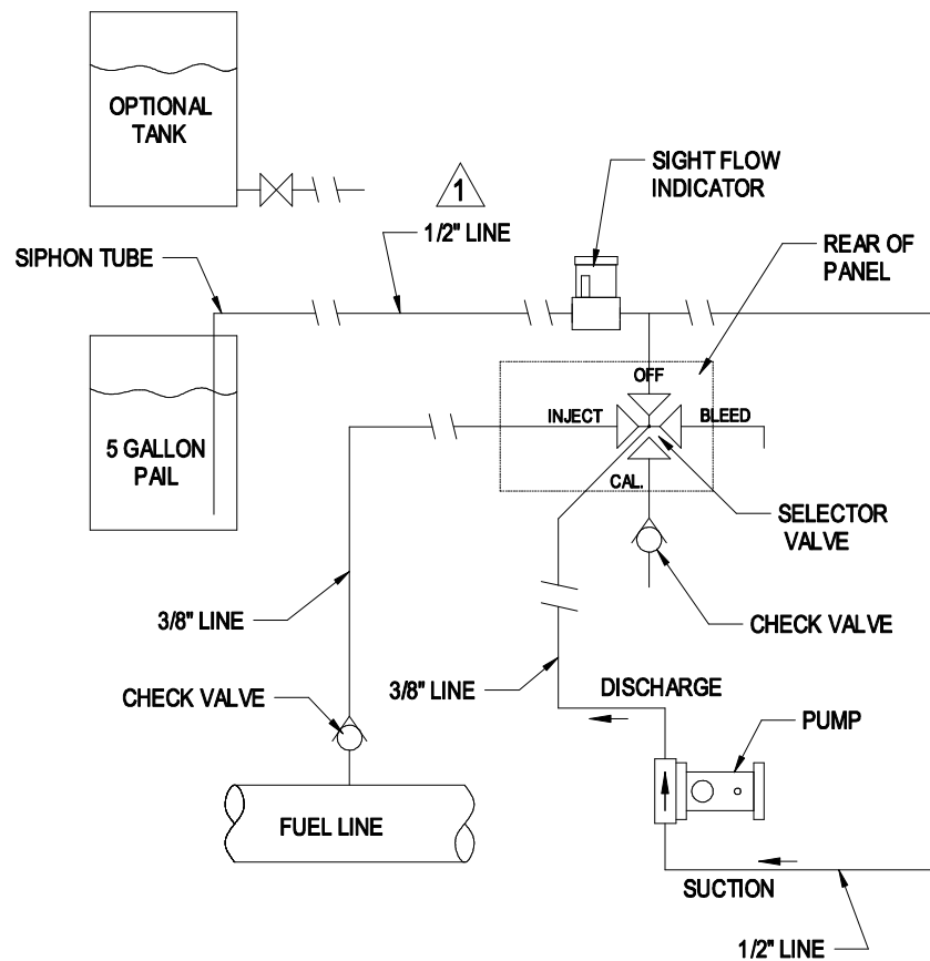
FLUID SCHEMATIC
