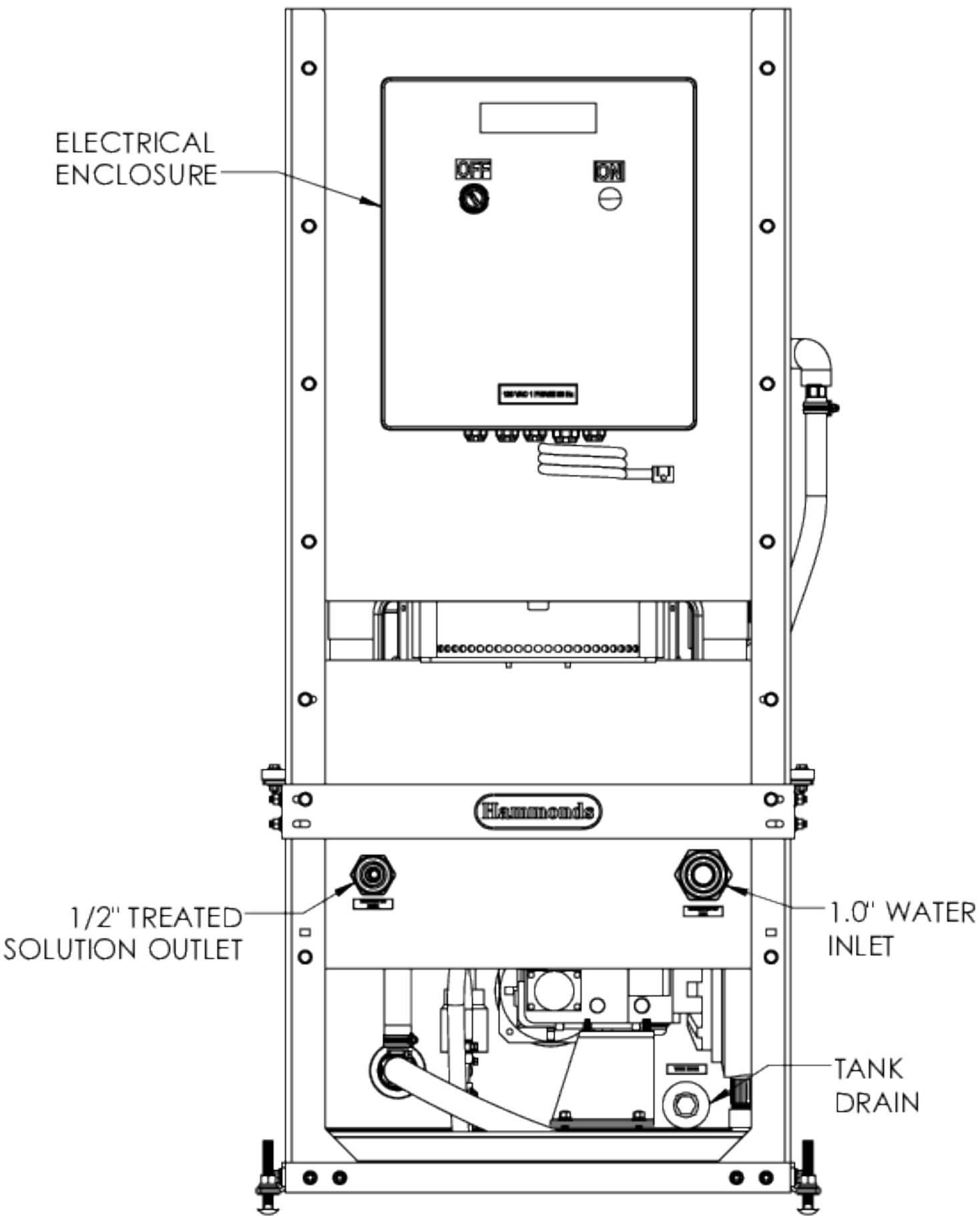
FRONT VIEW
